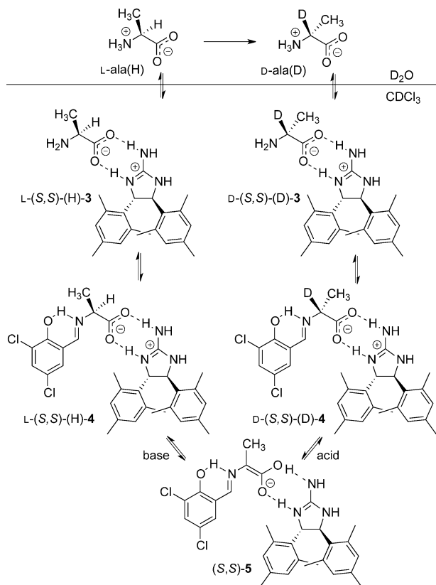
Scheme 2. Proposed mechanism for catalytic conversion of L -alanine to deuterated D -alanine.
