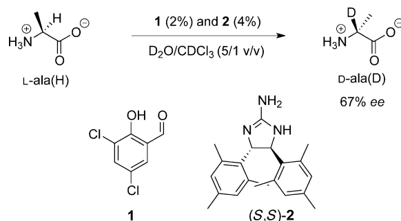
Scheme 1. Catalytic stereoselective deuteration of L-alanine to deuterated D-alanine using a pyridoxal analogue ( 1 ) and a chiral base ( 2 ).
