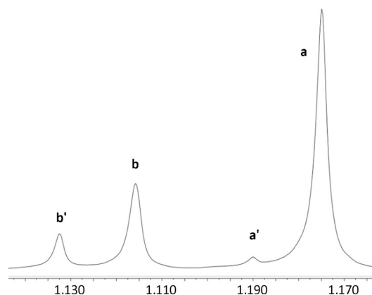
Figure 1. Signals in the 1 H NMR spectrum for the alanine salt methyl group after extracting the D 2 O layer with CDCl 3 as described in the text. a) Deuterated D-alanine salt. b) Deuterated L-alanine salt. b') Doublet signal of the initial non-deuterated L-alanine salt partially hidden under (b). a') Doublet signal of non-deuterated D-alanine salt partially hidden under (a).
