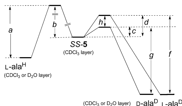
Scheme 3. Energy diagram for deuteration of L-ala H .
